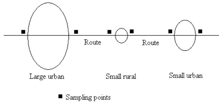
Figure 34: Sampling units
